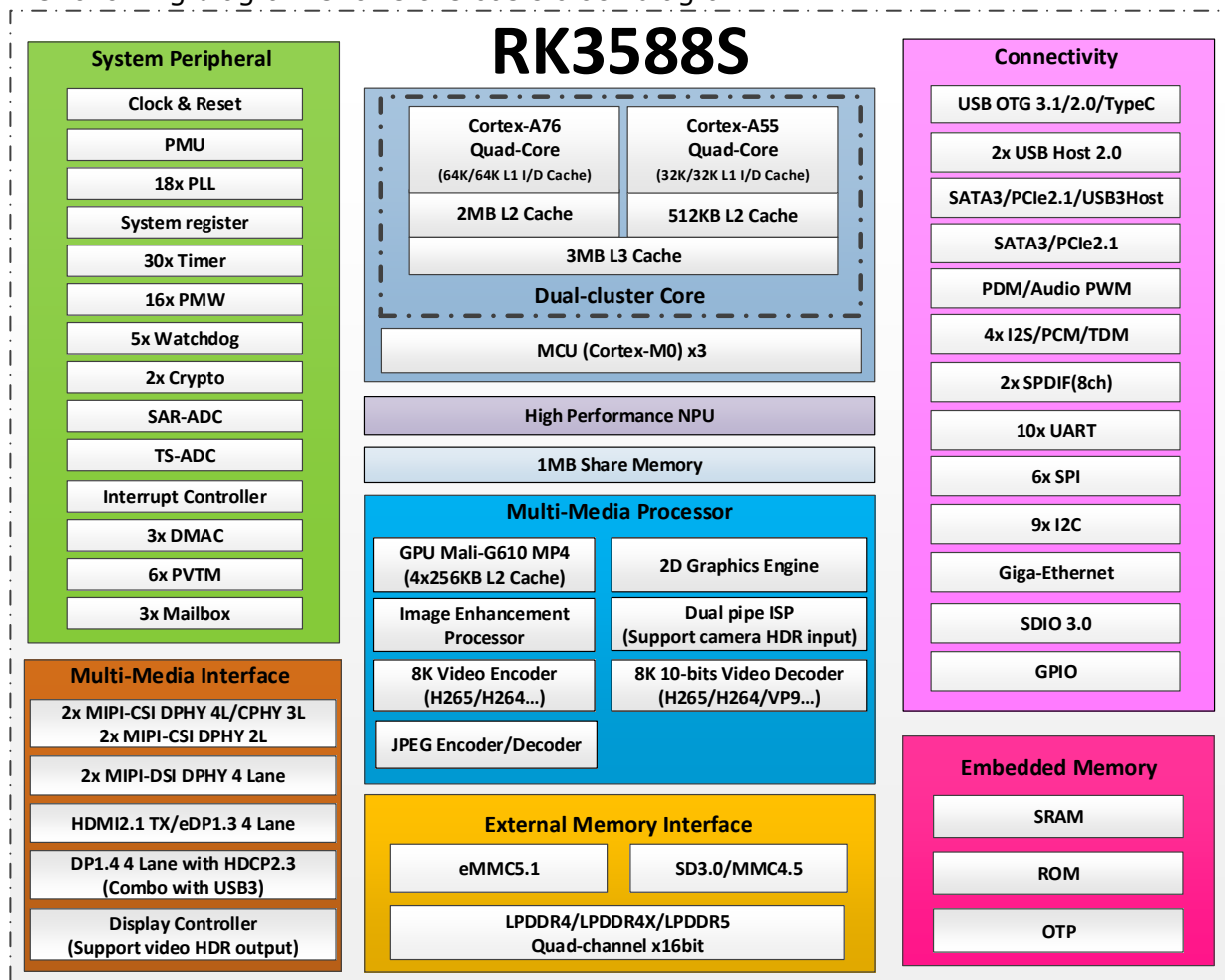
Fig.1-1 Block Diagram
