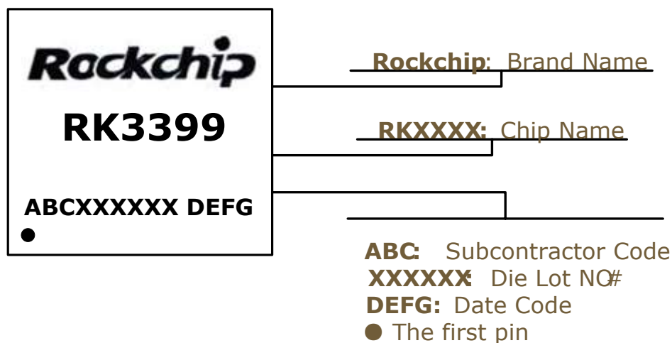
Fig. 2-1 Top Marking
