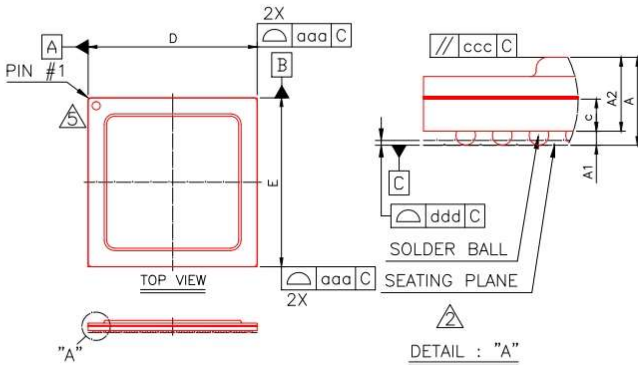
Fig. 2-2 Package Top and SideView
