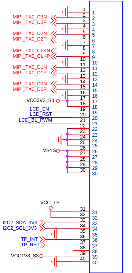
J2 FH34SRJ-30S 30_10P_FPC_BOT
