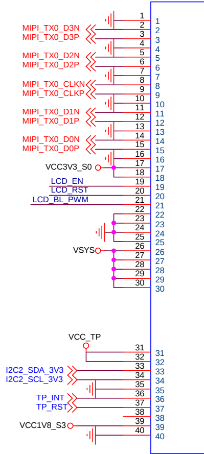
J3 FH34SRJ-30S 30_10P_FPC_TOP
